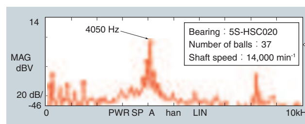
Fig. 8.12 Frequency characteristics of bearing noise (standard nozzle)
