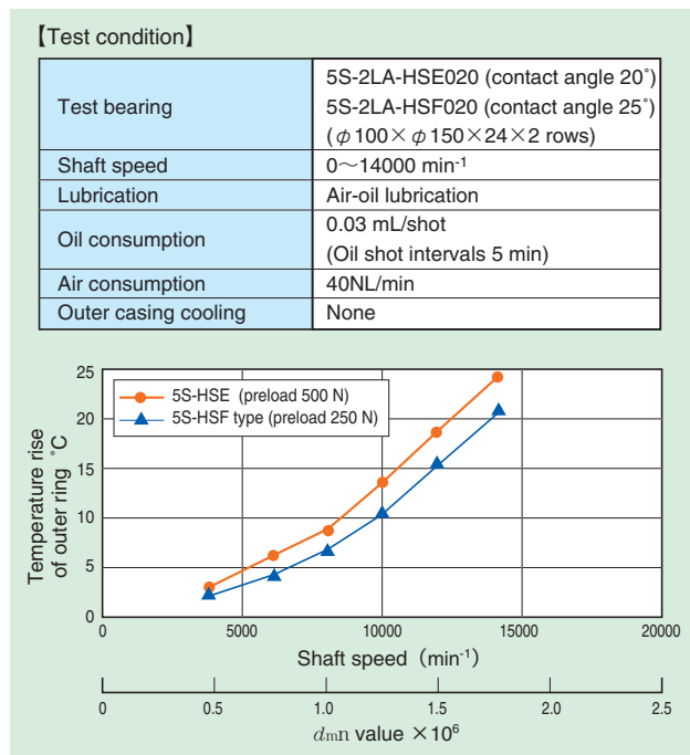
Fig. 9.27 Comparison of temperature rise
