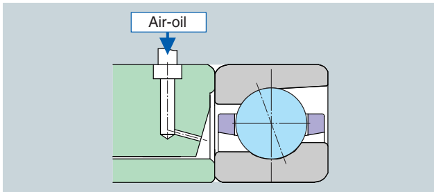
Fig. 9.20 79U and 70U types
