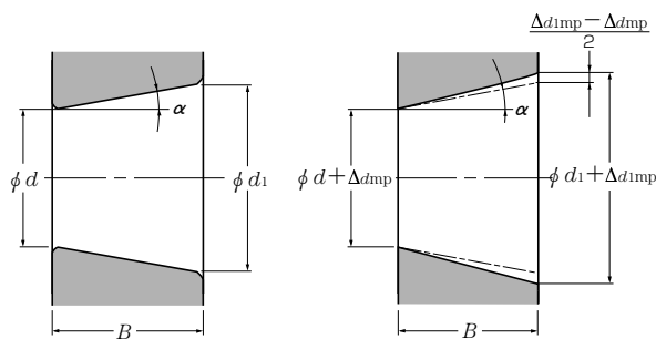
Theoretical tapered bore Tapered bore having single plane mean bore diameter deviation
