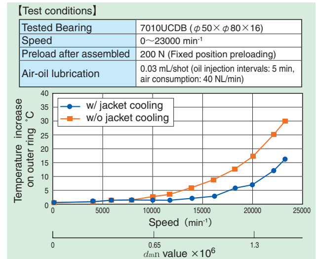
Fig. 9.22 High-speed test with air-oil lubrication
