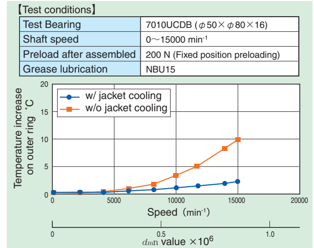
Fig. 9.21 High-speed test with grease lubrication
