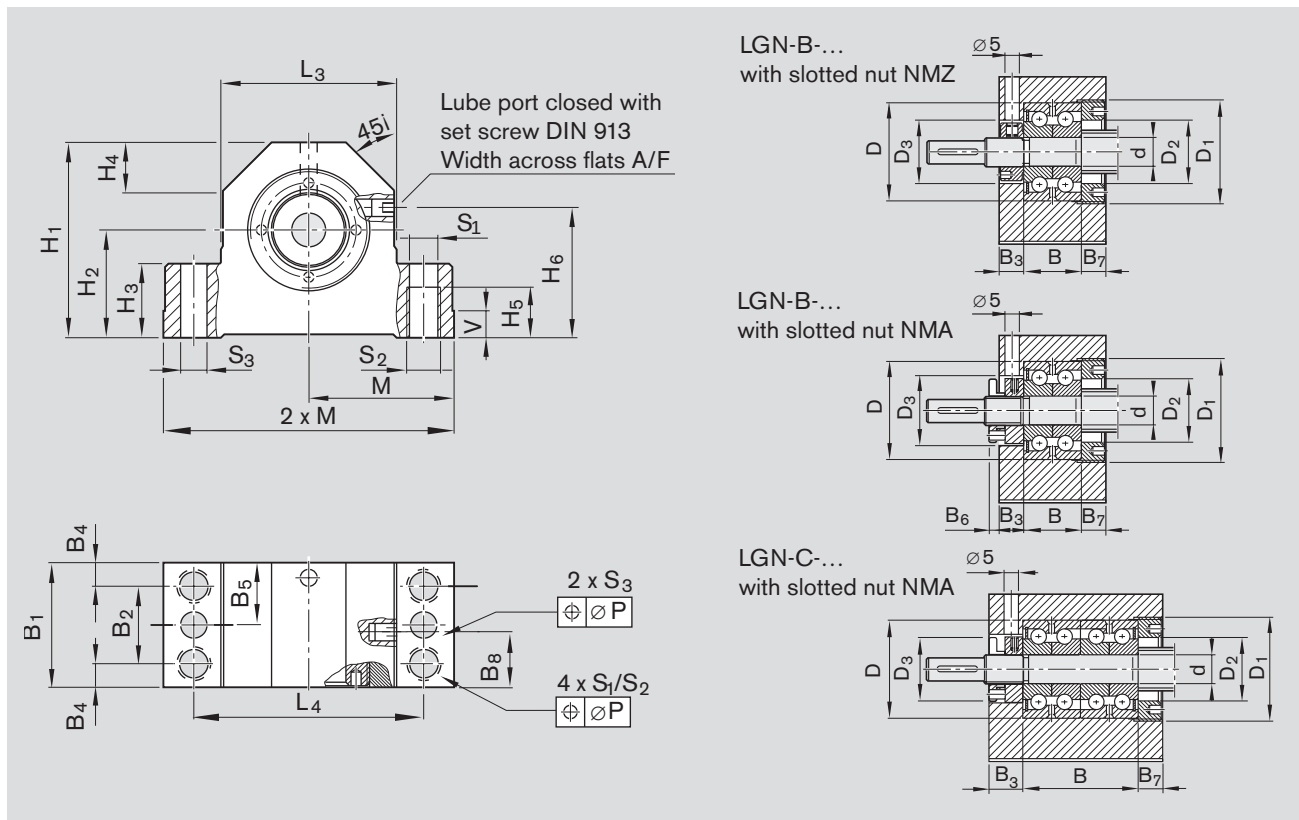
Dimensions (mm)
