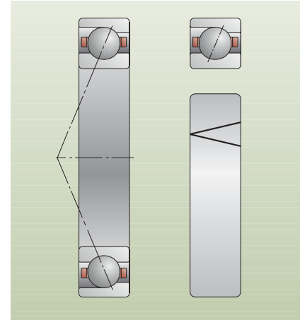
47: Contact angle marks on a single bearing
