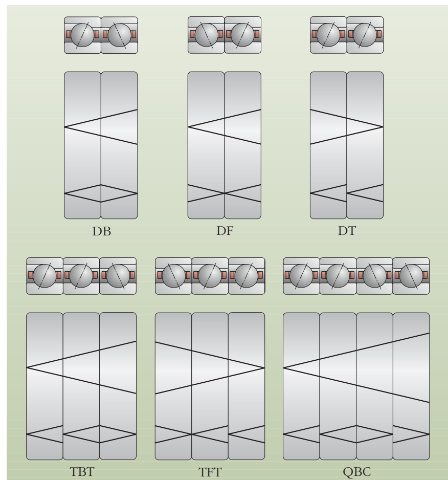
48: Examples of ready-to-mount bearing sets
