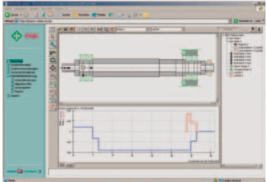
42: Calculation of the load distribution in a spindle
