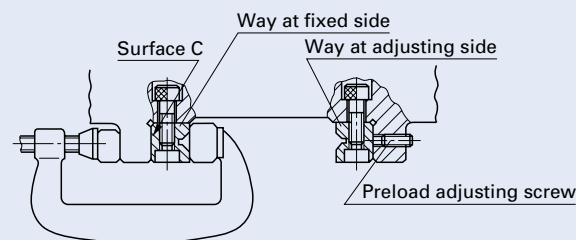
Fig. 16 Mounting of ways at table side (for Anti-Creep Cage Crossed Roller Way)
