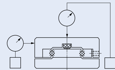
Fig. 19 Final checking of operating accuracy.
